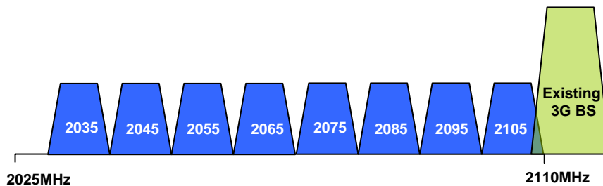
Figure 2: Current band plan and adjacency of 3G Base stations to Programme Making at 2110MHz
